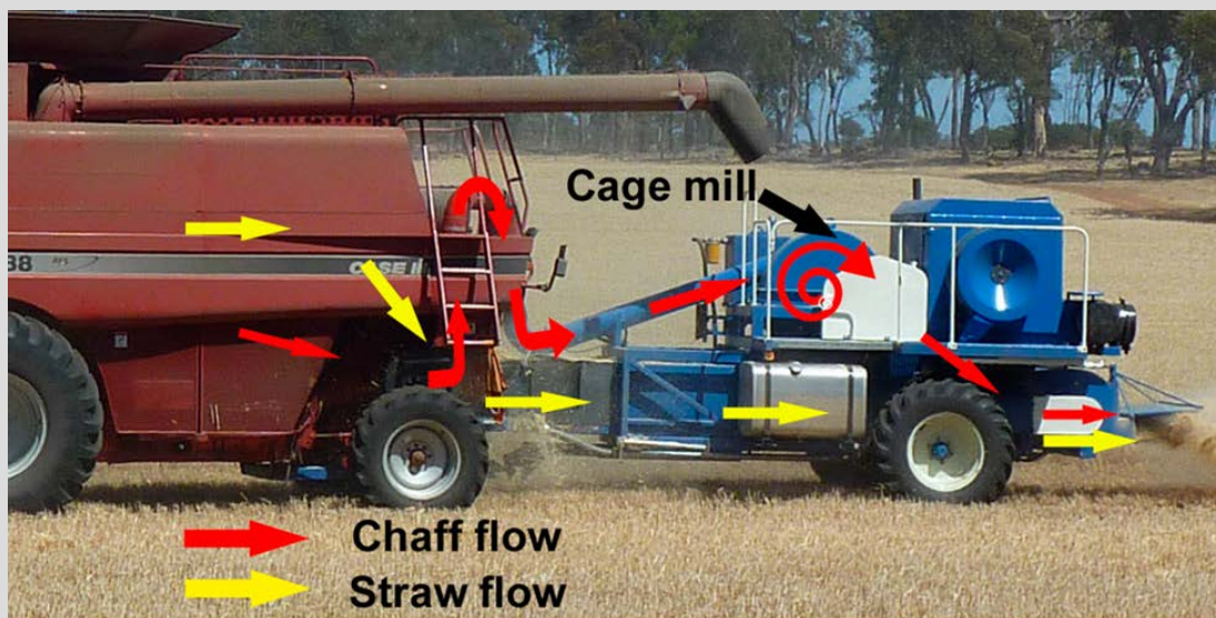
Photo 15.4. Flow of chaff and straw through the combine and the Harrington Seed Destructor.
